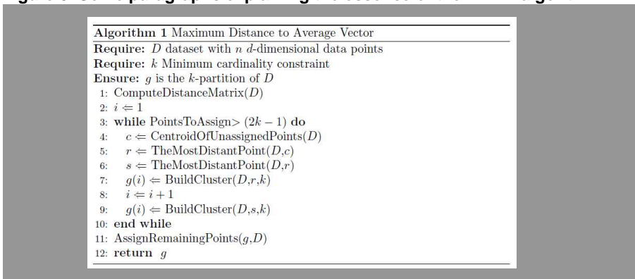
Figure 6. The MDAV explained using an algorithm.
