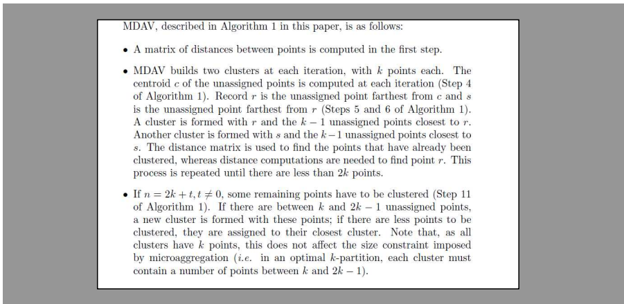
Figure 5. Some paragraphs explaining the essence of the MDAV algorithm.
