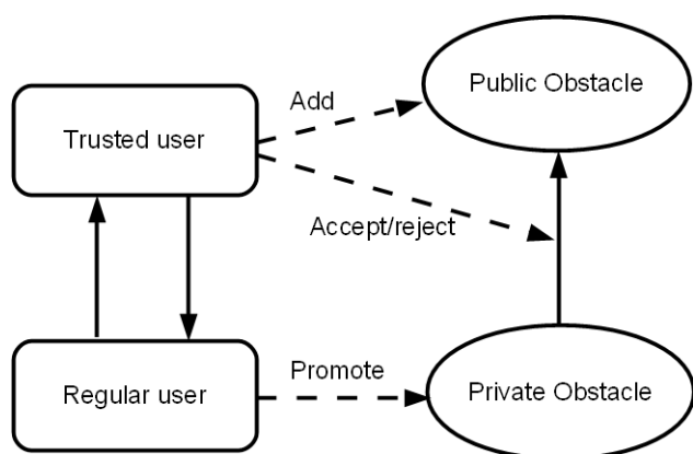
Fig. 9. Private data promotion
