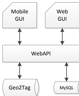
Fig. 7. “Accessibility map” architecture
